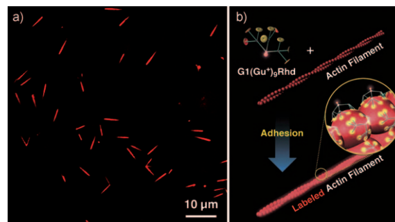
Figure 3. a) Confocal laser scanning micrograph of actin filaments in the presence of G1(Gu^+)_9Rhd (100 μM), upon excitation at 543 nm in a solution of KCl (100 mM) in HEPES buffer (20 mM, pH 7.0) with glucose (4.5 mg mL −1 ), catalase (0.036 mg mL −1 ), glucose oxidase (0.216 mg mL −1 ), and 2-mercaptoethanol (0.5 %). b) Illustration of a fluorescently labeled actin filament upon interaction with rhodamine-appended G1(Gu^+)_9Rhd .
